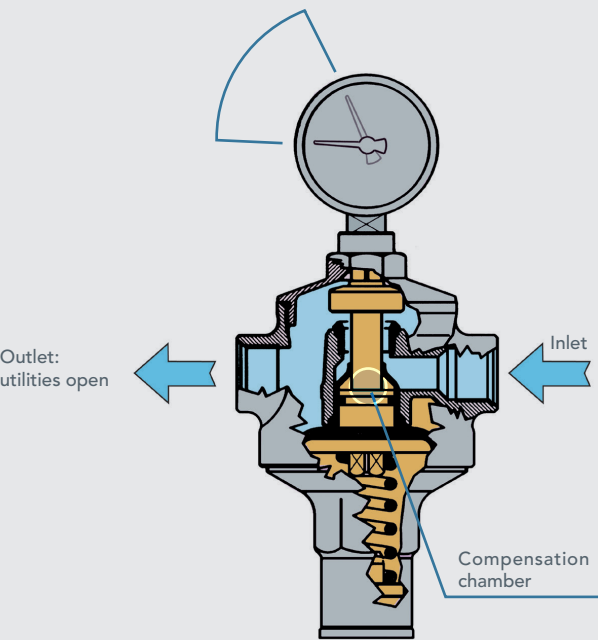
Pressure: P<3 bar
